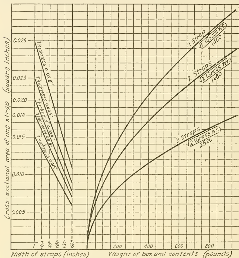
FIGURE 29.—Recommended sizes of flat metal straps for nailed boxes
